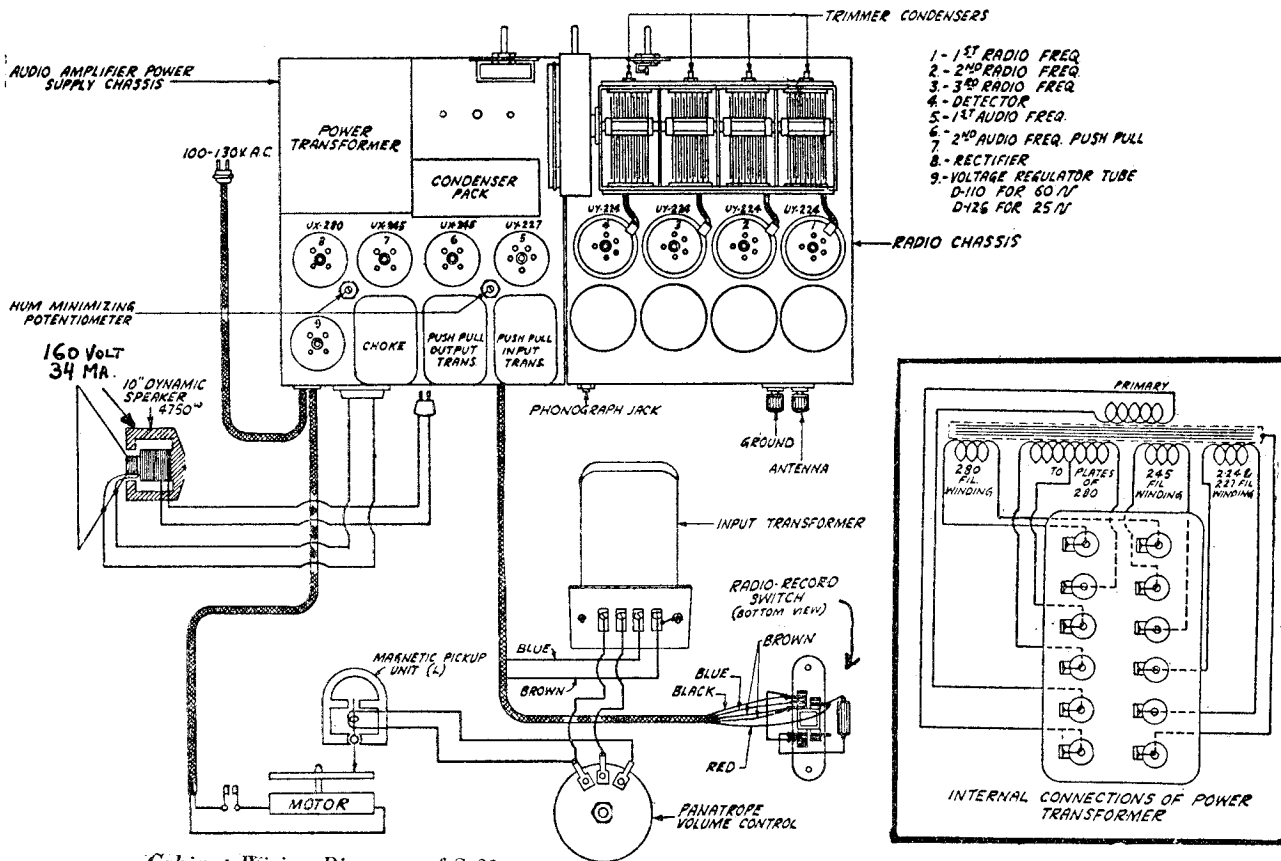
Cabinet Wiring Diagram of S-31
